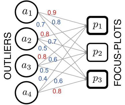
Fig. 3. LOOKOUT with k = 4 outliers, l = 3 focus-plots, and budget b = 2 : p_1 is picked first due to maximum total incrimination (sum of edge weights = 2.9); next p_3 is chosen over p_2 , due to its higher marginal gain (0.4 vs 0.2) (Color figure online)
